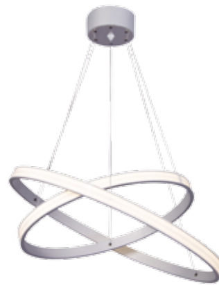
5300 ♂H57 aluminum Q LED 57,4W 3780 lm* 230 V Ø 64 cm ↓ max. 84 cm
