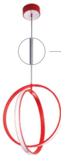
5204 ØH04 red Q LED 51,8W 3888 lm* 230 V Ø 48 cm ↓ max. 160 cm
